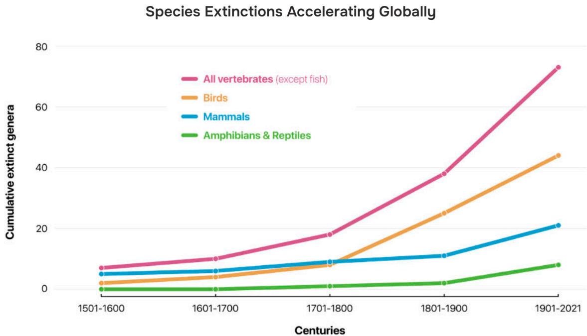
FIGURE 13 Species Extinctions Accelerating Globally. Cumulative number of genera extinctions per century in different classes of vertebrates. This graph shows that at least 73 genera have become extinct over the last 500 years. Similar estimates for mammals, birds, and fish indicate a total extinction rate of up to 100 E/MSY. 102 Data from Ceballos and Ehrlich, 2023. 95 Key takeaway: The significant and steadily increasing loss of global biodiversity raises concerns that Earth’s biosphere is losing resilience, adaptability and hence its ability to buffer against the different PB processes.
