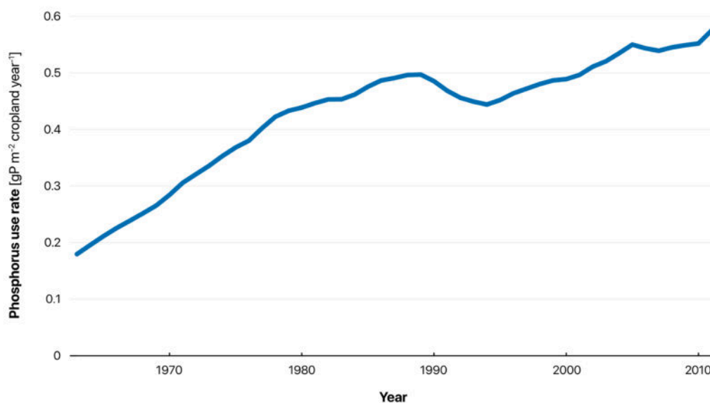
FIGURE 24 Rising Phosphorus Inputs for Agriculture. This graph shows the mean global phosphorus use rate on all croplands (in g P m -2 cropland year -1 , e.g., grams of phosphorus per square meter of cropland per year, see Supplementary Material ) from 1961 to 2013. Data from Lu and Tian, 2017. 130 Key takeaway: The rise in phosphorus use in agriculture is driving harmful algal and cyanobacteria blooms in freshwater systems, highlighting the urgent need for sustainable phosphorus management.
