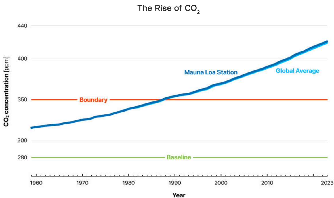
FIGURE 10 The Rise of CO 2 . This figure shows the annual global mean of atmospheric CO 2 concentration from 1979–2023, and the marginally different dataset of CO 2 concentration as measured at Mauna Loa in Hawaii, which integrates data over a longer timespan (from 1959–2023). The red line shows the PB of 350 ppm, while the green line represents the pre-industrial baseline of 280 ppm. CO 2 concentrations at Mauna Loa differ slightly from the global mean CO 2 value (with the former being approximately 2 ppm above the latter for recent years). Data from Lan et al., 2024 82 and Lan & Keeling, 2024. 86 Key takeaway: Atmospheric CO 2 concentrations have been continuously rising since industrialization and are now higher than at any time in the last 15 million years. 87
