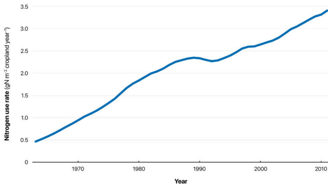
FIGURE 27 Rising Nitrogen Inputs for Agriculture. This graph shows the mean global nitrogen use rate on all croplands (in g N m -2 cropland year -1 , e.g., grams of nitrogen per square meter of cropland per year, see Supplementary Material ) from 1961 to 2013. Data from Lu and Tian, 2017. 130 Key takeaway: The steady increase in nitrogen use over the past decades reflects the growing use of nitrogen fertilizers to meet the demands of increasing agricultural production.
