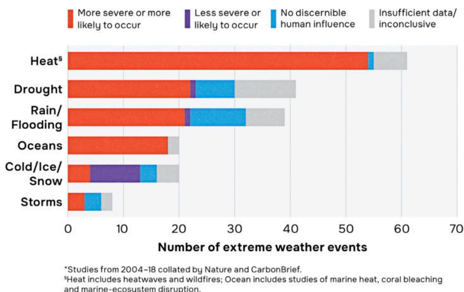
FIGURE 37 More Severe and More Likely - Extreme Weather Events Under Human-Induced Climate Change. An analysis of over 170 studies compiled by Nature and CarbonBrief shows that human-induced climate change has increased both the likelihood and severity of extreme weather events. Adapted from Schiermeier, 2018. 148 Reproduced with permission from Springer Nature. For an extensive and up-to-date overview of these numbers, refer to the latest attribution map of Carbon Brief (v2023). 133
