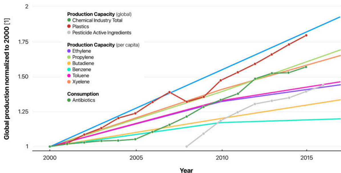
FIGURE 35 From Conception to Contamination: The Rise of Novel Entities. This chart illustrates the relative growth of various categories of novel entities and key chemicals from 2000 to 2017, a period with sufficient comparable data. The data is normalized to the year 2000. Data from Persson et al., 2022. 146 Key takeaway: Chemical production has steadily increased from 2000 to 2017, raising concerns about environmental contamination and public health. Novel entities, such as plastics, pesticides, industrial chemicals, and antibiotics, contribute to pollution, bioaccumulation, ecosystem disruption, antibiotic resistance, and health issues like cancer and hormonal imbalances. With tens of thousands of man-made chemicals in the world, most of which have not been studied for safety, the risks are significant.
