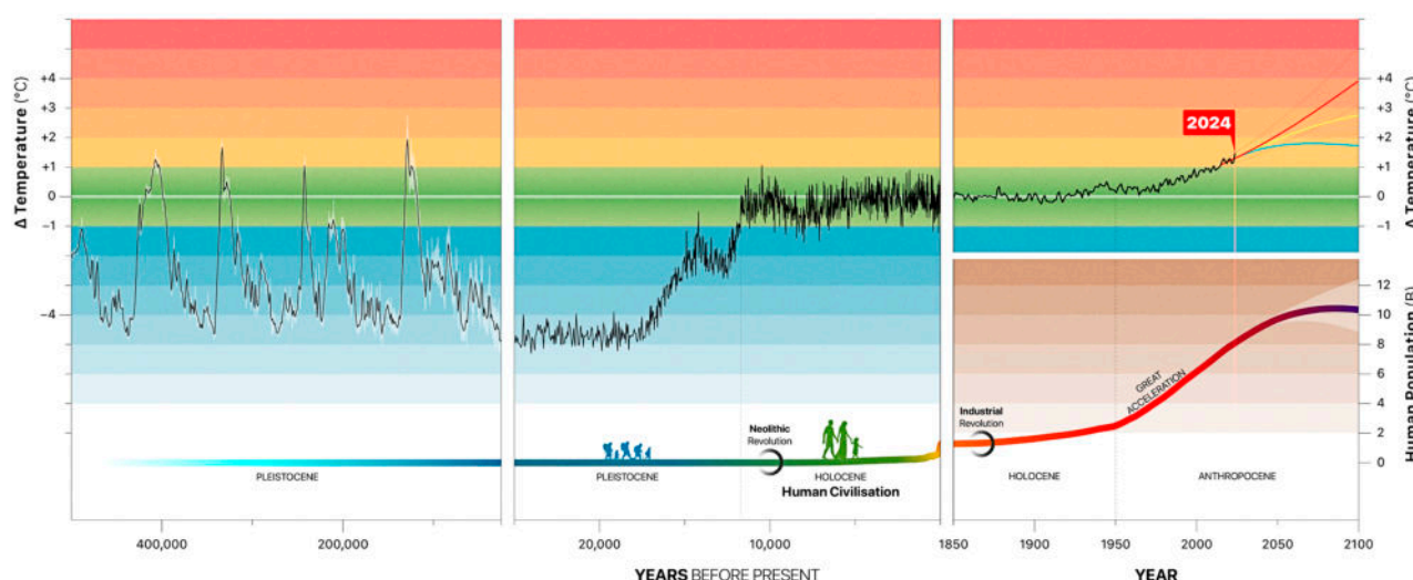
FIGURE 4 Humanity's Journey on Earth - Human Population Size and Global Temperature from 500,000 Years BP Until 2100. This figure is a composite of different data sets, including paleo data estimates, recent measurements, and future projections. For a detailed description of this figure, see Supplementary Material . Data from: Jouzel et al. 2007 7 , Masson-Delmotte et al. 2010 8 , Morice et al. 2021 9 , Osborn and Jones 2014 10 , CRU 2024 11 , IPCC Summary for Policymakers 2021 12 , Fyfe et al. 2024 13 , Ritchie et al. 2024 14 , Sjödin et al. 2012 15 , UN World Population Prospects 2022 16 . Key takeaway: For over 10,000 years, humanity lived in a very stable climatic period (the green corridor) in which it evolved and adapted its technologies and cultures. By crossing several Planetary Boundaries, including the one for Climate Change, this period has ended, and we are entering a new and dangerous terrain in which a still-growing world population must thrive.
