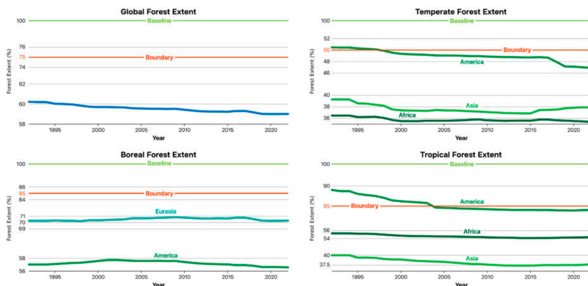
FIGURE 17 Global Forest Decline. Annual mean forest cover, expressed as a percentage of potential forest cover, globally and for three different biomes (temperate, boreal and tropical) between 1992 and 2022. Red lines show the Planetary Boundaries of 75%, 50%, 85% and 85% for global, temperate, boreal and tropical forests respectively, while the green line always represents the baseline of 100 % potential forest cover. Data from Copernicus, 2019 and Ramankutty and Foley, 1999. 104,105 Key takeaway: As a result of land-use and, increasingly, climate change, global and regional forests have been steadily declining over the last few decades across all major forest biomes. Most regions are already significantly below their regional boundaries, while some areas, such as temperate and tropical America, have just recently surpassed them.
