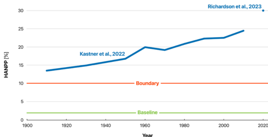
FIGURE 14 The Energy We Take From Nature and Use for Our Purposes. The plot displays the control variable "Human Appropriation of Net Primary Production (HANPP)," expressed as the percentage of the
