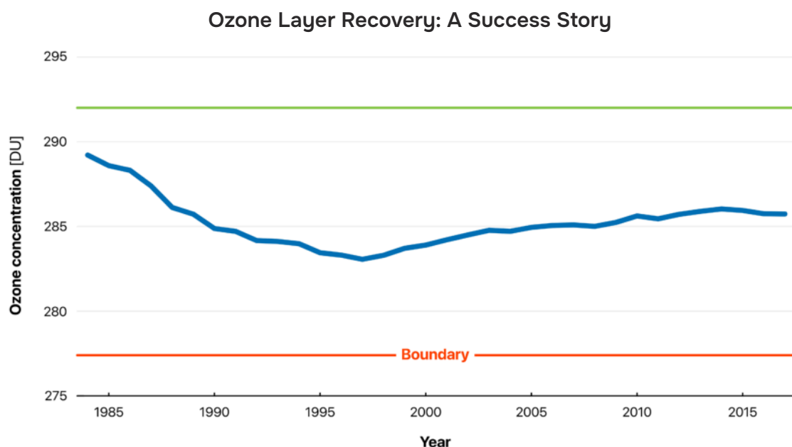
FIGURE 34 Ozone Layer Recovery: A Success Story. This chart displays the 11-year mean of the control variable “global mean stratospheric ozone concentration” measured in Dobson Units (DU) for the period from 1979 to 2022. The red line shows the Planetary Boundary of about 277 DU, while the green line represents the baseline of 292 DU (values updated with respect to Richardson et al., 2023 4 and IPCC, 2023 145 ). Data from MSR 2020. 140 Key takeaway: While the global stratospheric ozone layer has recovered since the mid-1990s after a significant decline, this recovery may have plateaued in recent years.
